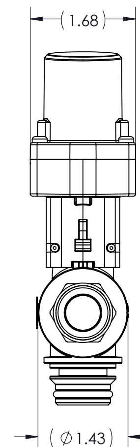
DETAIL A SCALE 2 : 1.5
