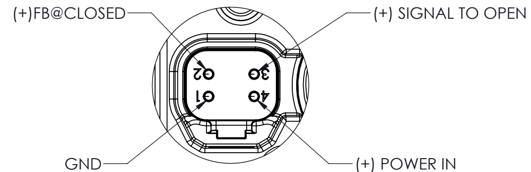
DETAIL A SCALE 2 : 1.5
