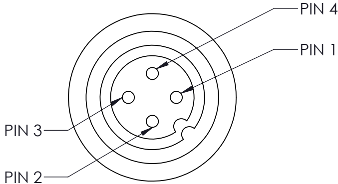
CONNECTOR END VIEW
